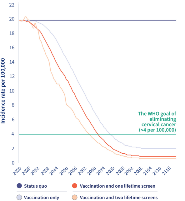
Figure 32.3 Global cervical cancer incidence rates under various scenarios of HPV vaccination and cervical screening, 2020-2120
